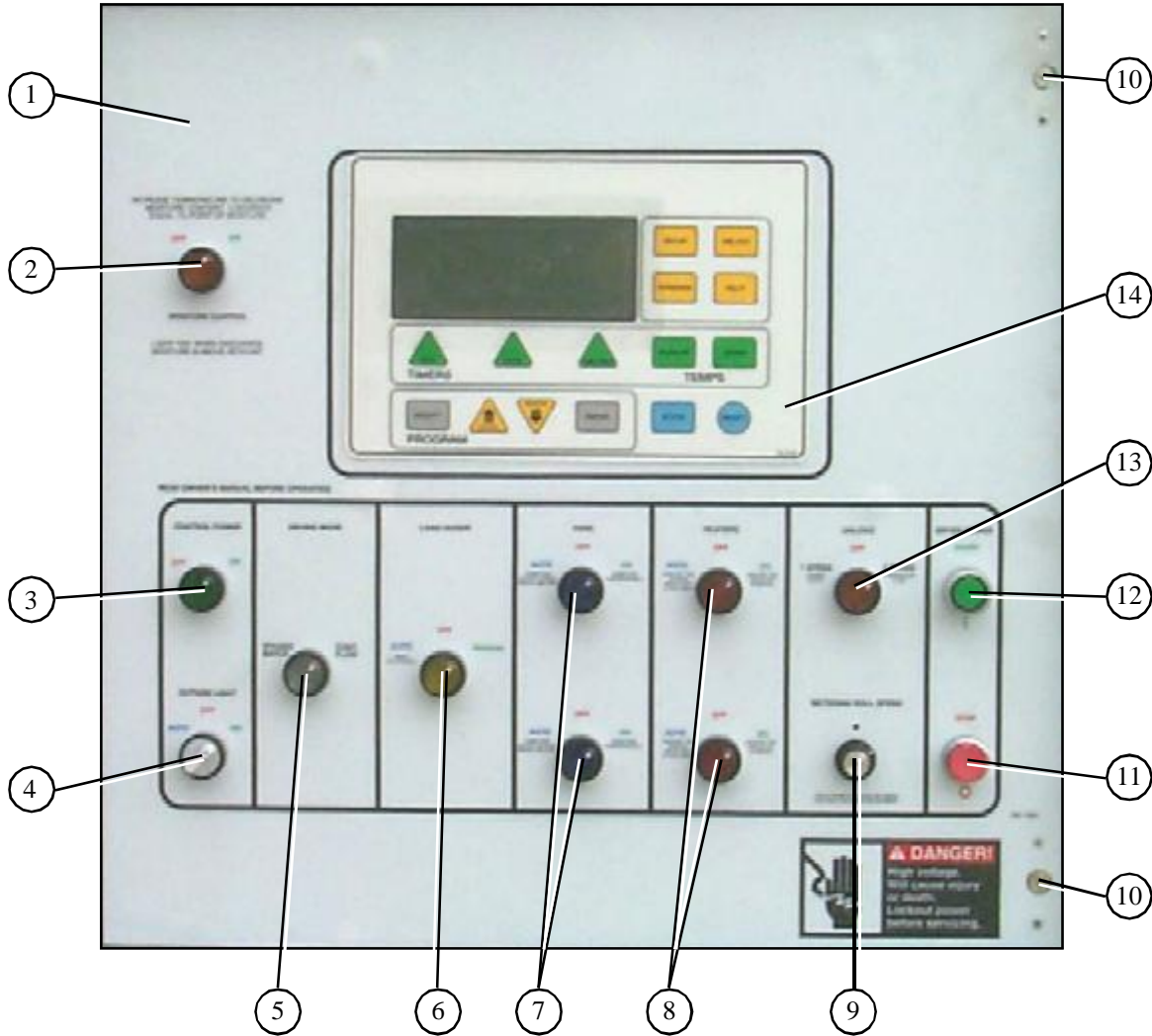
Network control panel (front).
